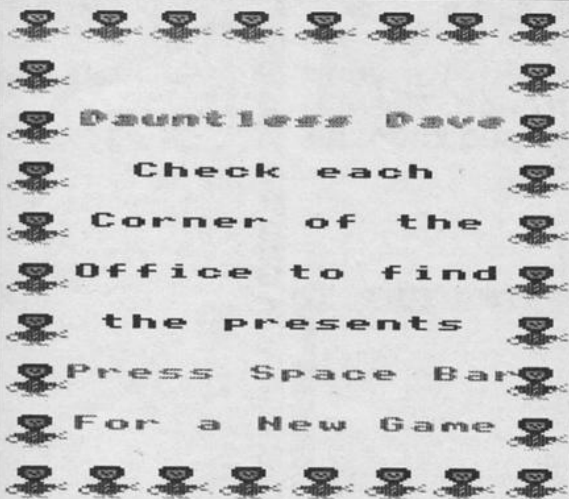
Screen dump
